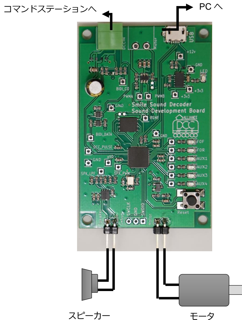
図 5.5.4.1 SmileSound Sound Development Board
